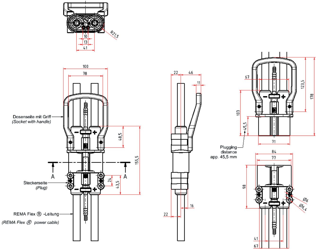
Plugging distance charts REMA® Electrical connector MRC 320
